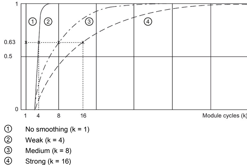
Figure 4-1 Smoothing with AI 4xI 2-/4-wire ST
