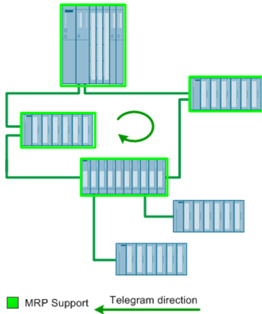
Figure 14-1 PROFINET with MRP
