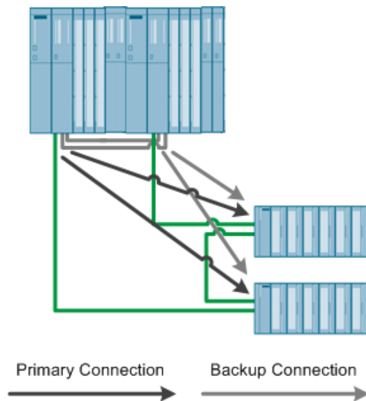
Figure 14-2 PROFINET with system redundancy
