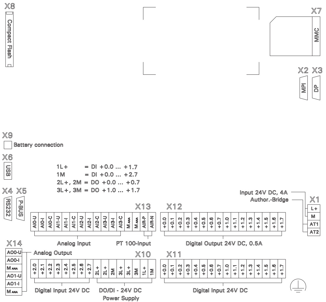
Figure 3-15 C7-636 imprint of connector pin assignment
