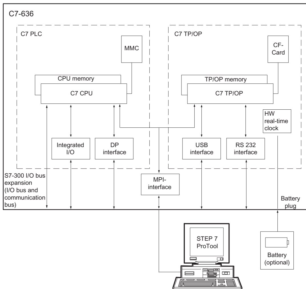
Figure 2-3 Components and interfaces of the C7-636
