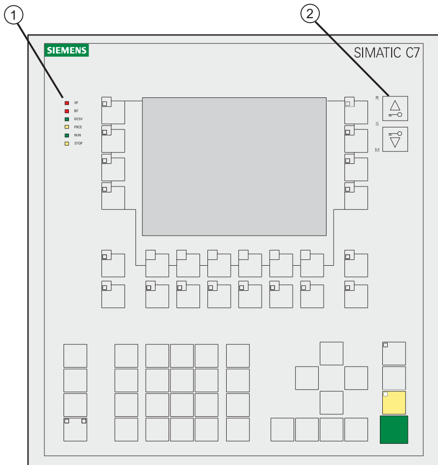
Figure 4-1 C7-636 Key
