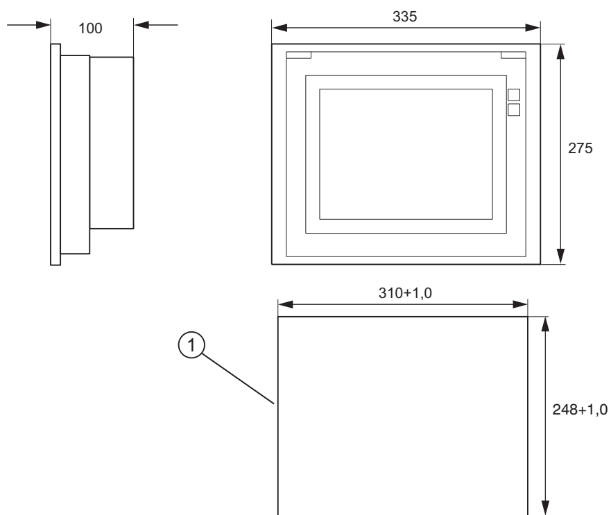
Figure 3-4 Dimension drawings for the C7-636 Touch (dimensions in mm)
