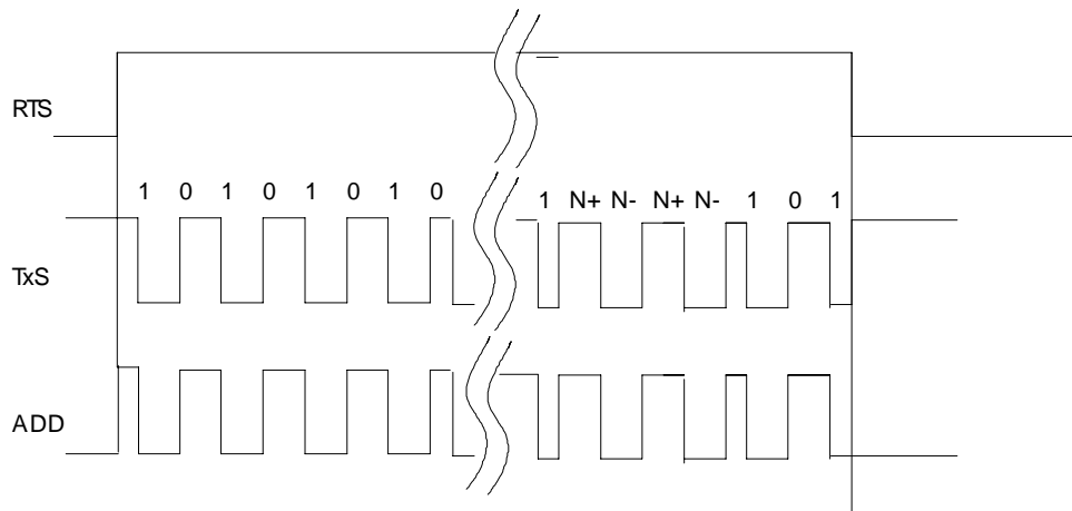
Figure 7.5-6: Output Signals of the Synchronous Transmitter
