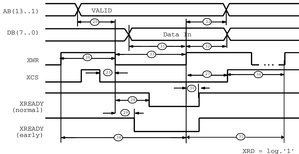
Figure 9.6-7: Asynchronous Intel Mode, Processor Write Timing
