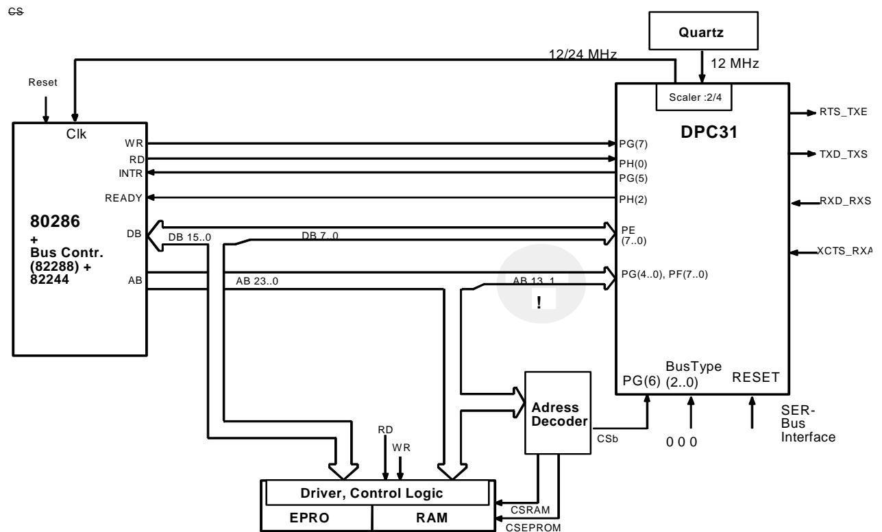
Figure 7.1-3: 80286 System as an Example for Mode X86
