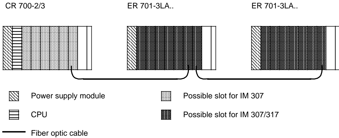
Figure 2-4. Basic Configuration with ER 701-3LA.. Expansion Subracks, with Interrupt Handling in the Expansion Unit
